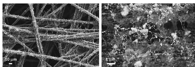
Fig. 5 SEM images of electrospayed 46 wt% Pt-CNT–C 6 H 5 PO 4 composites, showing direct contact between the electrolyte particles with the carbon nanotubes: (a) low and (b) high magnification.
