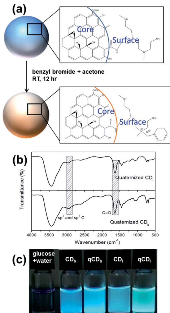
Fig. 5 (a) Illustration of the quaternization of PEI on the carbon dots. (b) FTIR spectra of the carbon dots quaternized with (a) branched PEI (CD b ) and (b) linear PEI (CD i ). (c) Optical images of (from L–R) glucose and water, CD b , quaternized CD b , CD i , quaternized CD i under UV lamp.
