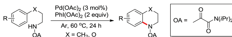
Scheme 444 Palladium-catalyzed intramolecular amination.
