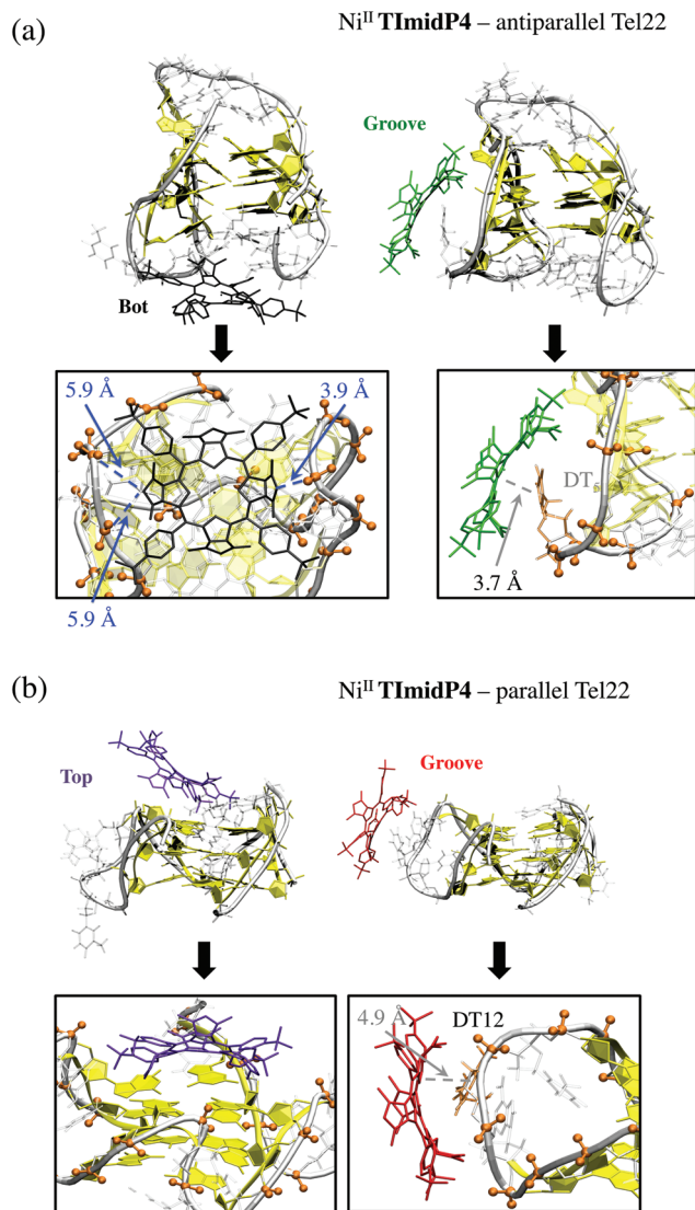
Fig. 5 Conformations and zooms of representative snapshots at the end of MD simulations of 1 : 1 Ni II -TmidP4 complex with (a) anti-parallel and (b) parallel G-quadruplexes. Porphyrins are coloured by binding modes ( i.e. , bot, top, and groove in black, violet and red/green, respectively). Relevant phosphates, residues are shown in orange. Relevant distances involving electrostatic and van der Waals interactions are shown in blue and grey, respectively.
