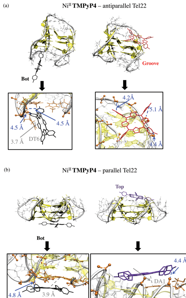
Fig. 6 Conformations and zooms of representative final snapshots from 100 ns MD simulations of 1 : 1 Ni II -TMPyP4 with (a) anti-parallel and (b) parallel G-quadruplexes. Porphyrins are coloured by binding modes ( i.e. , bot, top, and groove in black, violet and red, respectively). Relevant phosphates groups are coloured in orange. Relevant distances involving predicted electrostatic and van der Waals interactions are shown in blue and grey, respectively.
