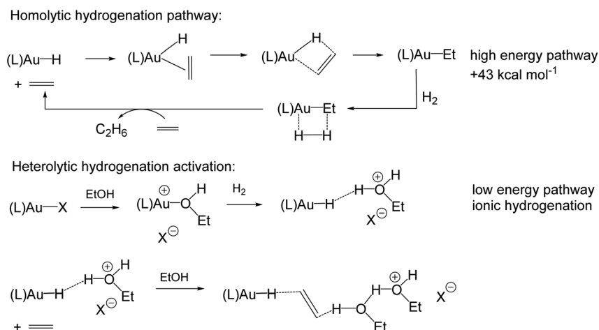
Scheme 6 Computational modelling of Au(i) mediated hydrogenation steps (L = IPPr).
