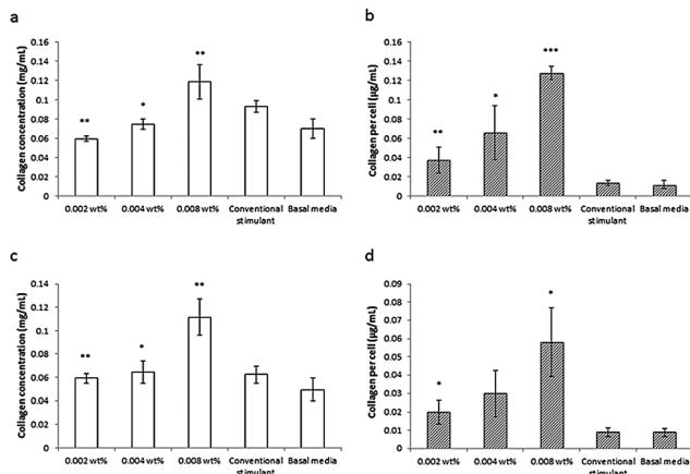
Fig. 17 Collagen assay results showing the stimulation of human fibroblasts by C_{16} -KTTKS. 81 (a) and (b) Human corneal fibroblasts, (c) and (d) human dermal fibroblasts. Left, total amount of collagen deposited by cells and right, total amount of collagen produced per cell ( n = 3 , *P \leq 0.005 , **P \leq 0.01 and ***P \leq 0.001 ).
