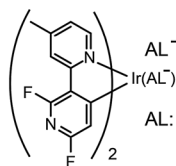
\text{Ir}[(\text{CF}_3)_2\text{Meppy}](\text{PPh}_3)_2(\text{H})(\text{NCMe})^+ 46
