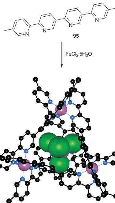
Fig. 16 The encapsulation of [\text{FeCl}_4]^- within a \text{Fe}_4(\mathbf{95})_6 cage, along with the crystal structure of \text{Fe}_4(\mathbf{95})_6 \cdot (\text{FeCl}_4) \cdot (\text{PF}_6)_7 \cdot \text{CH}_3\text{OH} . Iron and [\text{FeCl}_4]^- ions are shown in spacefill with ligand \mathbf{95} in ball-and-stick (iron: purple, chloride: green, nitrogen: blue, carbon: black). Hydrogen atoms, solvent molecules and counterions are omitted for clarity.
