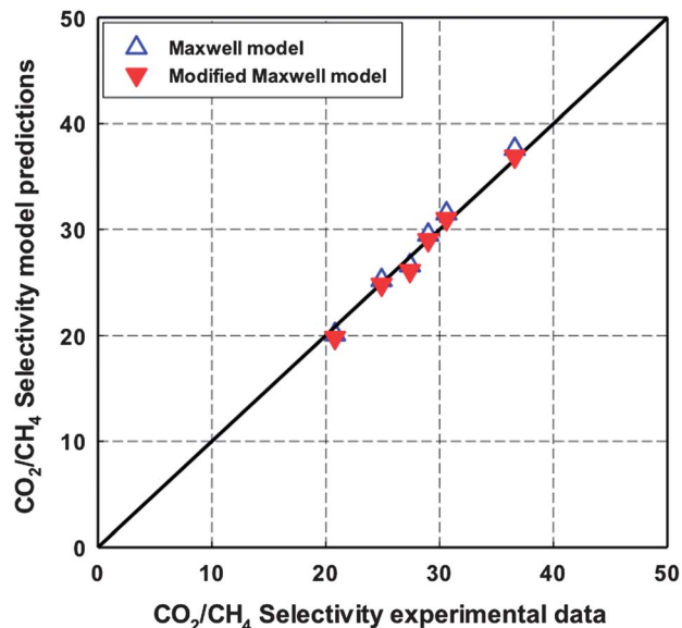
Fig. 16 Comparison of \text{CO}_2/\text{CH}_4 ideal selectivity of 6FOD(11) + 2%- \text{NH}_2 -MIL-53(Al) MMMs between experimental data and predictions from the Maxwell model and the modified Maxwell model.
