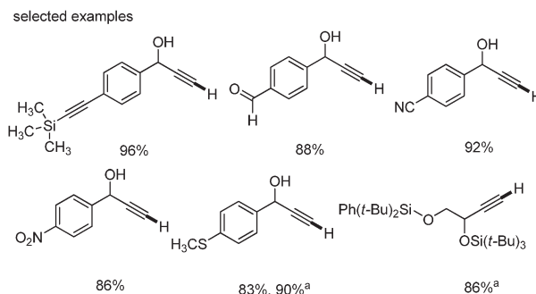
Scheme 54 Copper-catalyzed decarboxylation. a \text{Et}_3\text{N} 3.0 equiv. was used.
