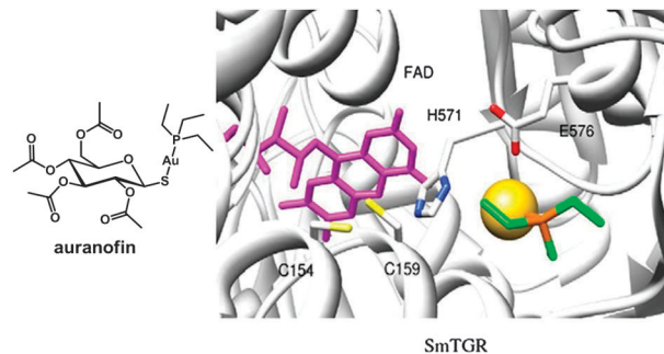
Fig. 11 Molecular structure of auranofin. Docked conformation of {Au(PEt 3 ) + truncated SmTGR. FAD is in violet sticks. The gold atom is a yellow sphere. Residues interacting with the gold atom are in sticks. Adapted from ref. 364.
