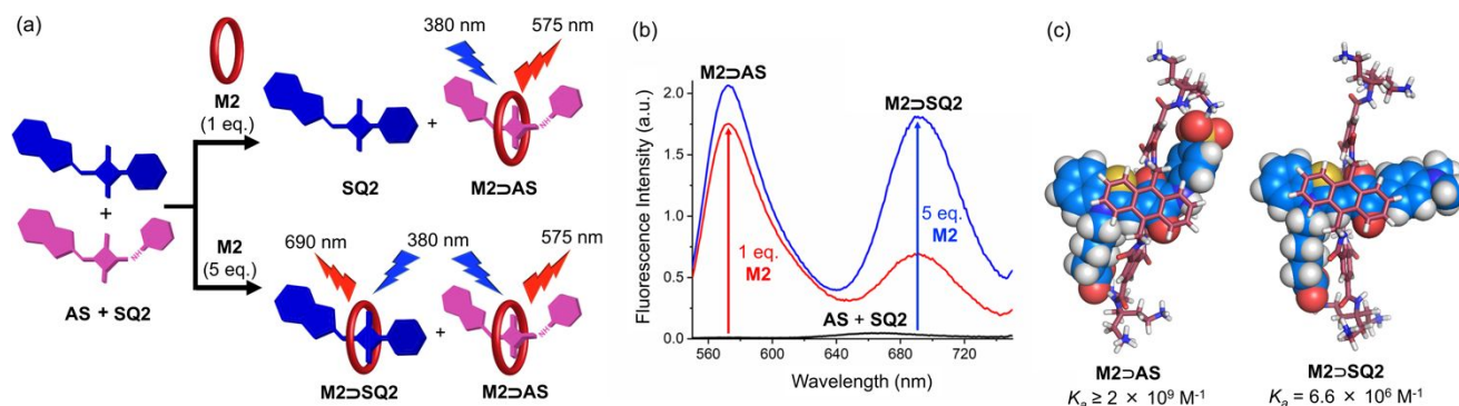
Figure 2. (a) Cartoon explaining the guest-selective encapsulation experiment. Addition of one molar equivalent (1 eq.) of M2 to a 1:1 binary mixture of AS and SQ2 selectively forms M2>AS , whereas addition of five molar equivalents (5 eq.) of M2 produces encapsulation of both guests. (b) Fluorescence profile for a binary mixture of 1:1 SQ2 and AS (2 \mu\text{M} each) with 380 nm excitation. Black curve: M2 is absent. Red curve: after one molar equivalent of M2 is added. Blue curve: after five molar equivalents of M2 is added. At 25 ^{\circ}\text{C} in PBS, pH 7.4. (c) Molecular models of energy-minimized complexes computed using the PM7 method.
