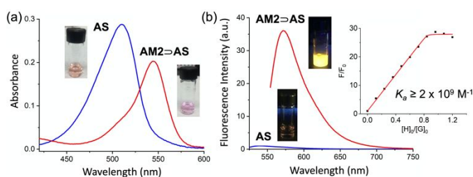
Figure 1. (a) Absorption spectra for AS (blue) and M2 ⊂ AS (red). (b) Emission spectra for AS (blue, ex: 510 nm) and M2 ⊂ AS (red, ex: 545 nm). In all cases, 10 \mu M in water at 25 °C. Insert: Representative titration isotherm with fitting to 1:1 association model.
