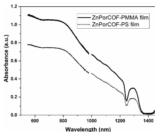
Figure 6. Absorption spectra for ZnPor-COF-polymer blends taken by integrating sphere, without scattering contributions. (We note that the lamp output ends at ca. 1400 nm; the dip at 1250 nm is likely related to overtone absorption losses by the optical fiber carrying the source light).
