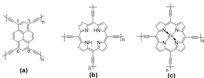
Figure 1. Chemical structures of the: (a) pyrene (Pyr-COF); (b) porphyrin (Por-COF); and (c) zinc porphyrin (ZnPor-COF) 2D COFs.
