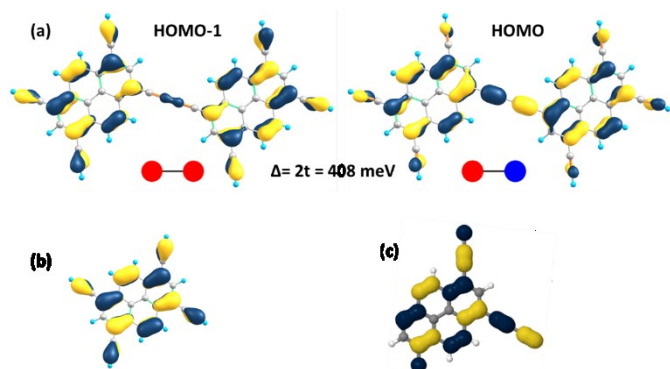
Figure 3. (a) Illustration of the HOMO and HOMO-1 wavefunctions in the Pyr-COF dimer and estimation of the transfer integrals ( t ) for holes, based on the energy-splitting approach; \Delta denotes the difference between the HOMO and HOMO-1 energies of the dimer; the red and blue dots express the symmetry of the tight-binding wavefunctions. (b) HOMO of the pyrene building block. (c) Wave-function of the valence band maximum of the 2D Pyr-COF at the \Gamma -point.
