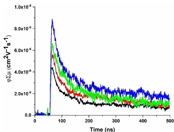
Figure 5. Representative fp-TRMC transients with increasing fluence ( 1 \times 10^{14} - 4 \times 10^{15} photons \text{cm}^{-2} ) for a ZnPor-COF-PS film at 700 nm photoexcitation with 7 ns pulse width.
