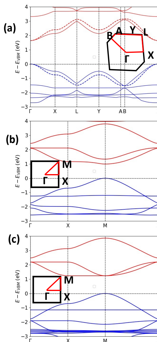
Figure 2. DFT-PBE0-calculated electronic band structures of: (a) Pyr-COF (the two bands depicted with dashed lines refer to those derived from the tight-binding modelling); (b) Por-COF; and (c) ZnPor-COF (the Brillouin zones and high-symmetry points are shown in the insets). The valence and conduction bands are colored in blue and red, respectively. The zero of energy is taken as the valence band maximum, E_{\text{VBM}} (shown by the horizontal dashed gray line).
