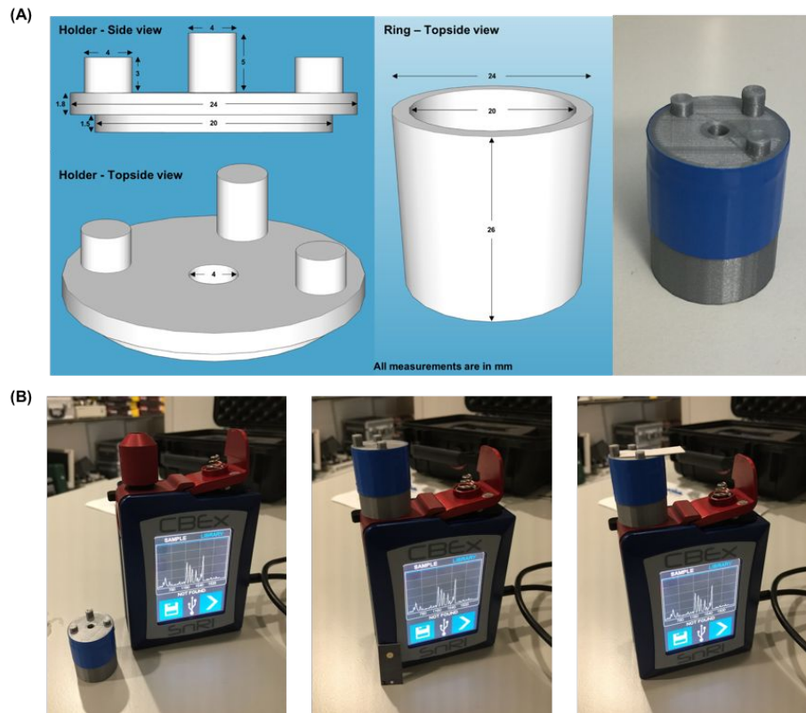
30 31 32 33 34 35 36 37 38 39 40 41 42 43 44 45 46 47 48 49 50 51 52 53 54 55 56 57 58 59 60 Figure 2. (A) shows the design and dimensions of the Raman aperture adaptor used for the analysis of the capture layer contained within the 3-D paper device. The adaptor was appropriately scaled to ensure that readouts were made at the optimal distance and center of the spot (B) Images display how the adaptor fits over the point and shoot lens and how the capture layer is mounted to enable SERS analysis.
