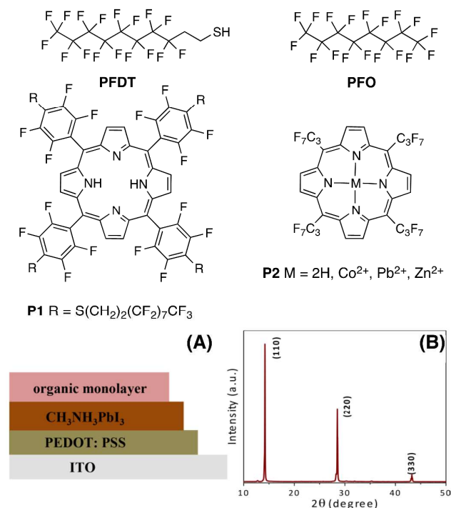
Fig. 1 Structure of fluorinated derivatives, (A) architecture of devices for Kelvin probe studies, and (B) characteristic tetragonal phase XRD pattern of MAPI samples used.
