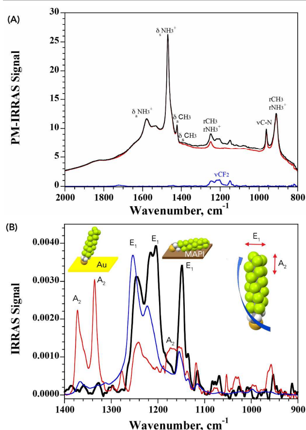
Fig. 3 (A) PM-IRRAS spectra of pristine MAPI (red line) and after exposure to PFDT (black line). The baseline-corrected difference signal evidencing the CF 2 vibrations is shown in blue. (B) IRRAS spectra of PFDT on MAPI (black line) vs. gold (red line). The blue line corresponds to the simulated spectrum of a 5 Å-thick isotropic layer of PFDT . The helical conformation of perfluoroalkanes results in vibrational transitions grouped either vertically ( A_2 , along the helix axis) or horizontally ( E_1 ), allowing the molecular orientation with respect to the substrate to be assigned as shown.
