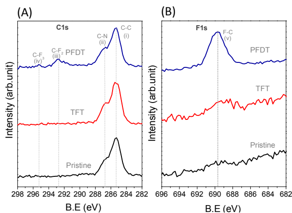
Fig. 2 XPS spectra of (A) C 1s, and (B) F 1s from pristine perovskite, TFT and PFDT passivated perovskite surface. Peak assignments (i) C-C (285.3 eV), (ii) C-N (286.7 eV), (iii) C-F (-CF 2 ) (292.8 eV), (iv) C-F (-CF 3 ) (295.1eV), and (v) F-C ( 689.7 eV).
