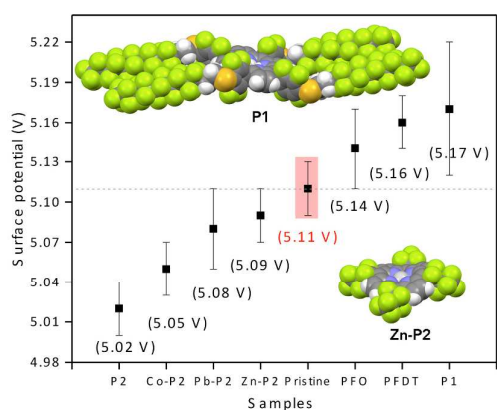
Fig. 5 Surface potential determined from triplicate Kelvin probe measurements of pristine MAPI and following formation of monolayers with P1 and P2 . The solid-state
