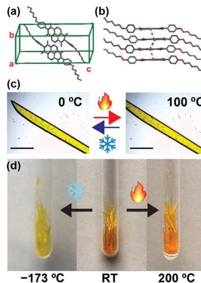
Figure 4. (a) Unit cell packing structure of HxNDI, (b) alternating interplanar distances of HxNDI (c) POM images showing HxNDI single crystal expansion during heating from 0 °C to 100 °C (Scale Bar is 500 μm), and (d) thermo-chromic behaviour of HxNDI.
