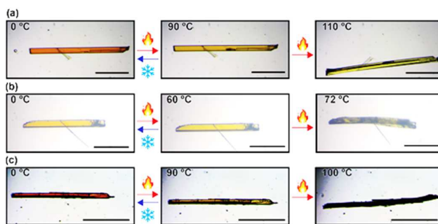
Figure 3. Thermo-chromic and thermo-mechanical properties of (a) HNDI, (b) ONDI, and (c) NNDI. First two images in a sequence show thermo-chromic behaviour (if any) and the final, irreversible step shows the product of the thermo-salient behaviour—typically the crystal splits. Scale bar is 500 μm.
