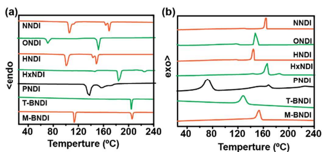
Figure 1. (a) Heating curves of ANDI derivatives and their corresponding (b) cooling curves. Orange lines correspond to monoclinic crystal systems and green lines correspond to triclinic crystal systems.
