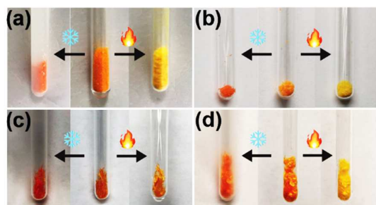
Figure 5. Thermochromic behavior of (a) PNDI, (b) HNDI, (c) ONDI, and (d) NNDI. All the samples were heated to 100 °C and cooled to -173 °C for the visualization of thermochromic behavior.
