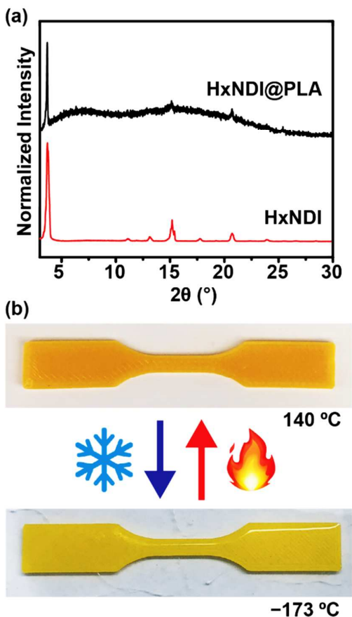
Figure 7. (a) PXRD data for HxNDI@PLA composites and (b) positive thermochromic behavior of HxNDI @PLA.
