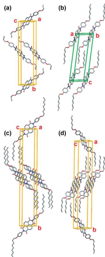
Figure 2. Comparison of thermo-salient derivative unit cells: (a) BNDI-M (b) ONDI and (c) NNDI (d) HNDI. Orange unit cell axes correspond to monoclinic crystal systems and green unit cell axes correspond to triclinic crystal systems.
