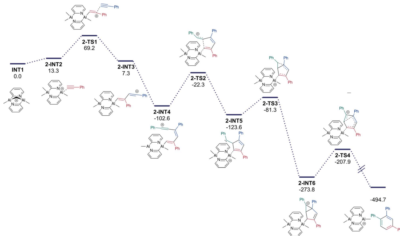
Fig. 13 Proposed reaction mechanism and energy profile diagram of the calculated trimerisation reaction pathway (Gibbs free energies in kJ mol -1 ).
