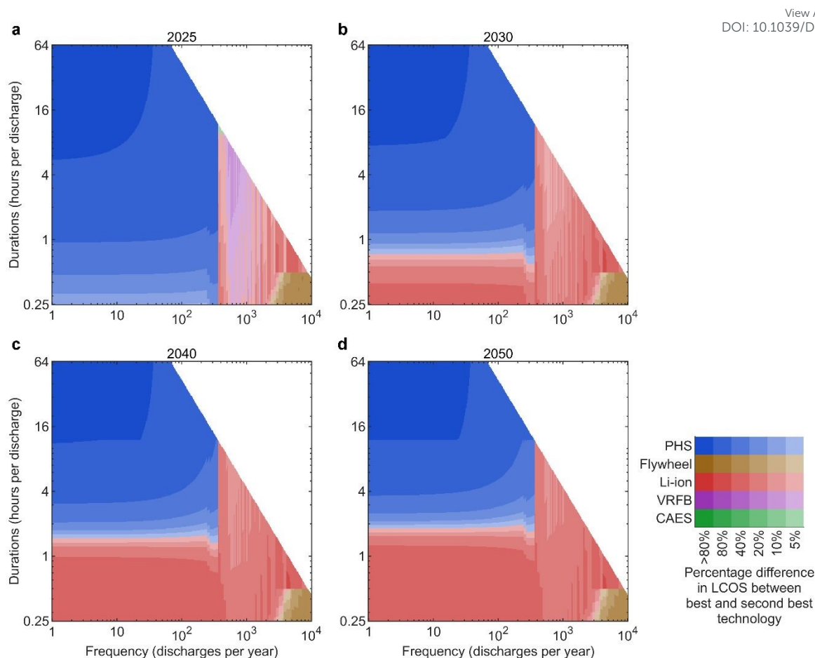
Fig. 2. Cost competitiveness of energy storage technologies across discharge duration and cycling frequency from 2025 to 2050. (a) 2025 cost benchmark. (b) 2030 cost benchmark. (c) 2040 cost benchmark. (d) 2050 cost benchmark. Each panel shows the technology with the lowest LCOS under a given combination of discharge duration and annual cycling frequency. Colors indicate the percentage cost difference between the most competitive technology and the second-best option.
