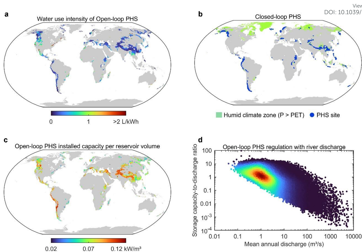
Fig. 5. Hydrological constraints and storage-flow relationships of PHS. (a) Water usage to offset evaporation and seepage per unit electricity generated by open-loop PHS. (b) Global distribution of closed-loop PHS sites constrained to humid climate regions where long-term precipitation exceeds potential evaporation ( P > PET ). (c) Installed open-loop PHS capacity per unit reservoir volume. (d) Ratio of PHS reservoir storage volume to mean annual river discharge of the host river basin. Gray regions indicate areas without PHS resources.
