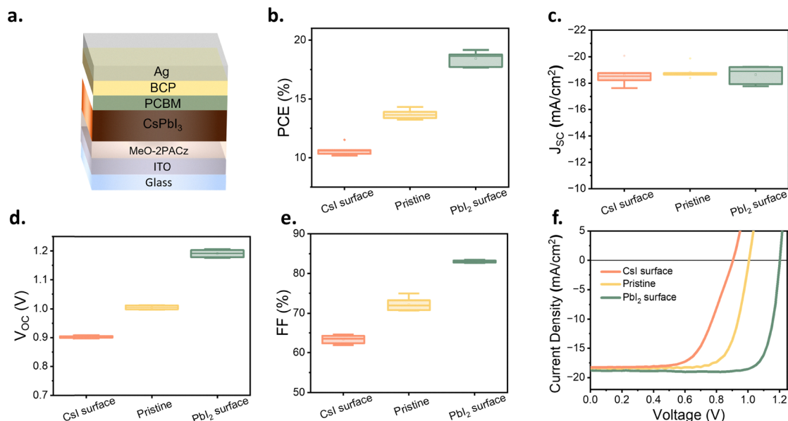
Fig. 2 Photovoltaic performance of treated CsPbI 3 . (a) Architecture of PV device. (b) PCE distribution, (c) J_{SC} distribution, (d) V_{OC} distribution, (e) FF distribution, (f) J - V characteristics of treated CsPbI 3 solar cells. The box plots in panels (b)–(e) display the mean, median line, 25%–75% box limits with 1.5\times interquartile range whiskers. The total number of samples is 18. The corresponding values in panels (b)–(e) are provided in the Table S1. The forward and reverse scans of f are provided in the Fig. S3.
