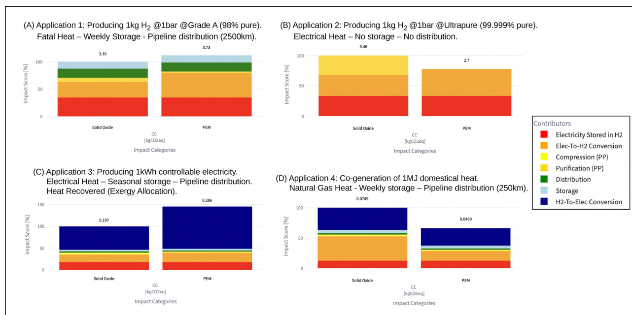
Fig. 7 Comparative LCA of solid oxide and proton exchange membrane systems for various scenarios. Impact scores (IW + expert version) are computed with the HTWOL and are normalized to the solid oxide system results. The contribution of each life cycle stage is represented, using the same colors as the framework representation.
