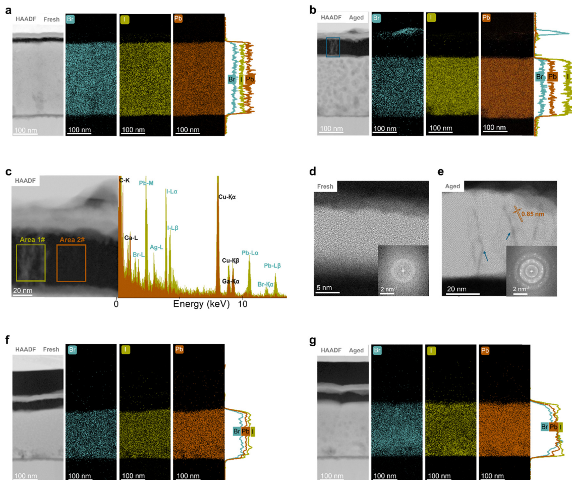
Fig. 4 Cross-sectional STEM and EDXS characterization. (a) and (b) Cross sectional STEM-HAADF images and the corresponding EDXS maps of Br, I, and Pb of fresh and aged SPVK, respectively. (c) The zoom-in area of flocculent-like features in the aged C_{60} film and the corresponding EDX spectra extracted from two marked areas, i.e. , area #1 from flocculent-like features region and area #2 from its neighbouring region without the flocculent-like feature as seen from the corresponding STEM-HAADF image. Noted that the y axis scale of the EDX spectrum represents the counts of X-ray photons. (d) and (e) STEM bright-field images of C_{60} films of freshly prepared and aged SPVK devices, respectively, with the FFT images as insets. (f) and (g) Cross-sectional STEM-HAADF images and the corresponding EDXS maps of Br, I, and Pb of fresh and aged P-Q TSCs, respectively.
