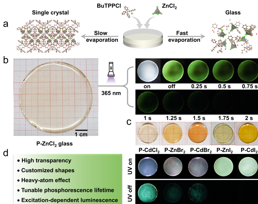
Fig. 1 (a) Schematic diagram of illustrating the controllable synthesis of \text{P-ZnCl}_2 glass and crystal via the solvent-assisted rapid and slow evaporation method. The left side shows the crystal structure of \text{P-ZnCl}_2 single crystal, and the right side shows the amorphous molecular structure of \text{P-ZnCl}_2 glass. (b) Photographs of \text{P-ZnCl}_2 glass with a diameter of 6 cm under ambient light, UV irradiation (365 nm), and UV off. (c) Photographs of \text{P-CdCl}_2 , \text{P-ZnBr}_2 , \text{P-CdBr}_2 , \text{P-ZnI}_2 , and \text{P-CdI}_2 glasses under ambient light, UV irradiation (365 nm), and UV off. (d) The typical features of the (\text{BuTPP})_2\text{MCl}_2\text{X}_2 glasses.
