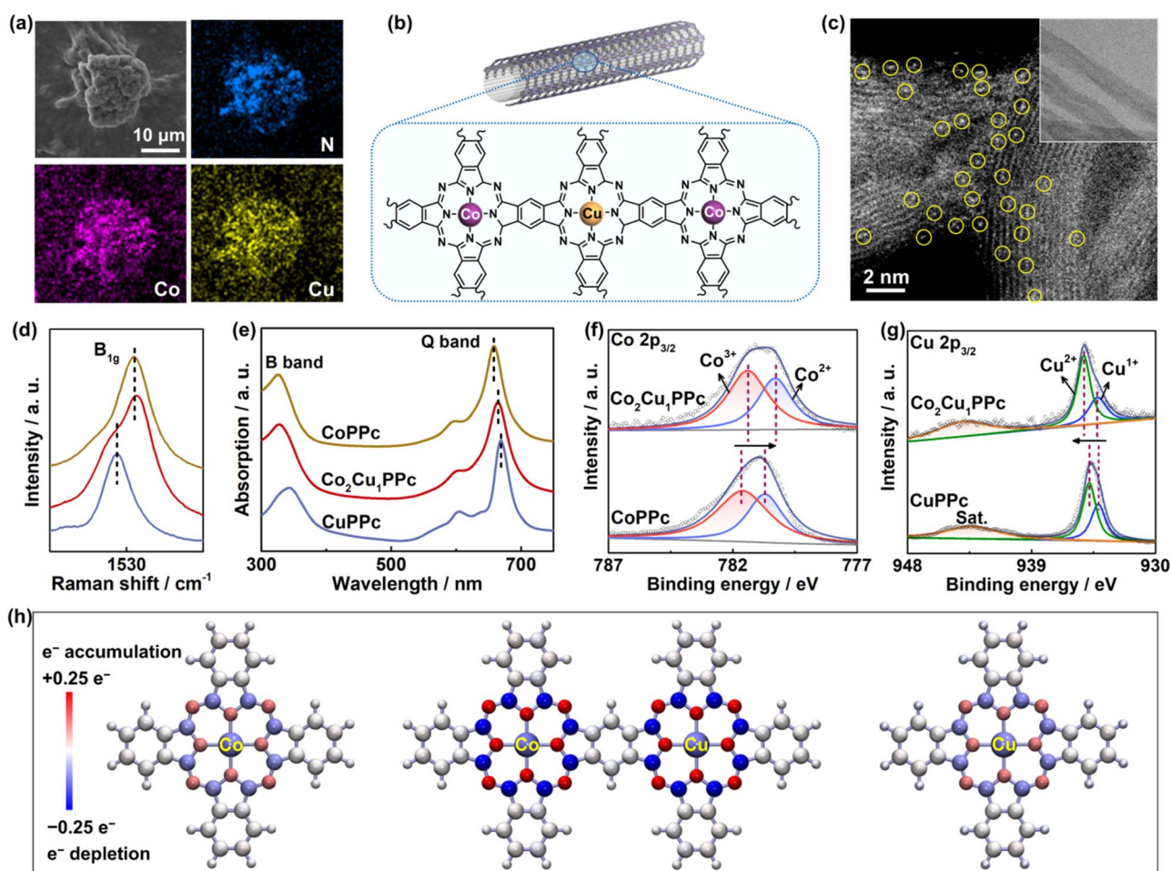
Fig. 1 Material characterization. (a) SEM and EDS mapping of unsupported \text{Co}_2\text{Cu}_1\text{PPc} . (b) Schematic diagram of \text{Co}_2\text{Cu}_1\text{PPc} supported on CNTs. (c) Atomic-resolution HAADF-STEM images of \text{Co}_2\text{Cu}_1\text{PPc} supported on CNTs (circled bright spots represent the metal atoms; inset: HRTEM). (d) Raman and (e) UV-Vis spectra of unsupported CoPPc, \text{Co}_2\text{Cu}_1\text{PPc} and CuPPc. High-resolution XPS spectra of (f) Co 2p_{3/2} and (g) Cu 2p_{3/2} of CoPPc, \text{Co}_2\text{Cu}_1\text{PPc} and CuPPc. (h) Bader charge analysis of CoPc, CuPc and simplified heteronuclear \text{Co}_2\text{Cu}_1\text{PPc} (the red and blue colors represent accepting and losing electrons, respectively).
