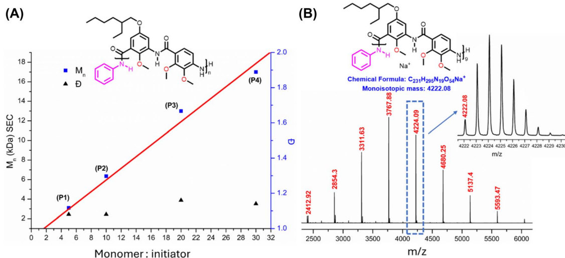
Fig. 6 (A) Linear plot of observed M_n vs. M_2 : I_1 ratio for the synthesis of polymers P1 to P4 . (B) MALDI-ToF mass spectrum (DCTB, NaTFA) of P2 matching with the proposed end groups.
