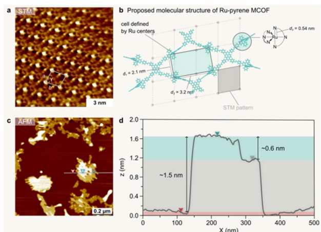
Fig. 15 Scanning probe microscopies characterisation of the Ru-pyrene MCOF. (a) High-resolution STM image showing the Ru-pyrene MCOF imaged at the heptanoic acid/HOPG interface. The measured distances and angle between repeating units obtained from calibrated STM images are: a = 1.7 \pm 0.1 nm; b = 1.8 \pm 0.1 nm; \gamma = 80 \pm 3^\circ . Imaging parameters: V_{\text{bias}} = -0.4 V, I_{\text{set}} = 150 pA. (b) Molecular models of the Ru-pyrene MCOF and Ru-metalloligand 3 (inset). Relevant intramolecular and intralayer distances between Ru atoms are given in nm. The STM pattern is overlaid in grey. (c) AFM image showing the layered morphology of the Ru-pyrene MCOF. (d) Line profile across one of the islands in (c) showing the step height of ca. 0.6 nm. Reproduced from ref. 67 with permission from Wiley-VCH, copyright 2025.
