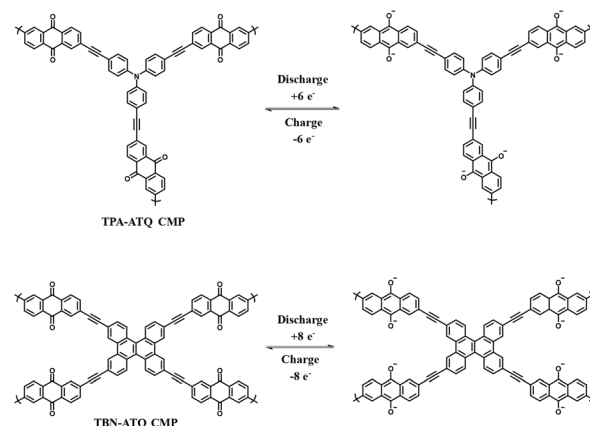
Fig. 21 Reversible redox-mechanism of TPA-ATQ CMP and TBN-ATQ CMP.
