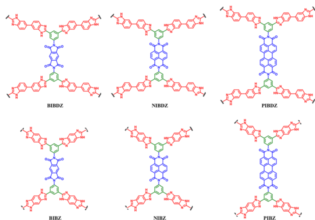
Fig. 40 Porous cross-linked polymer structures of benzimidazole-linked arylimide constituted from 3,3'-diaminobenzene (DAB) and (b) 1,2,4,5-benzenetetraine (TAB).
