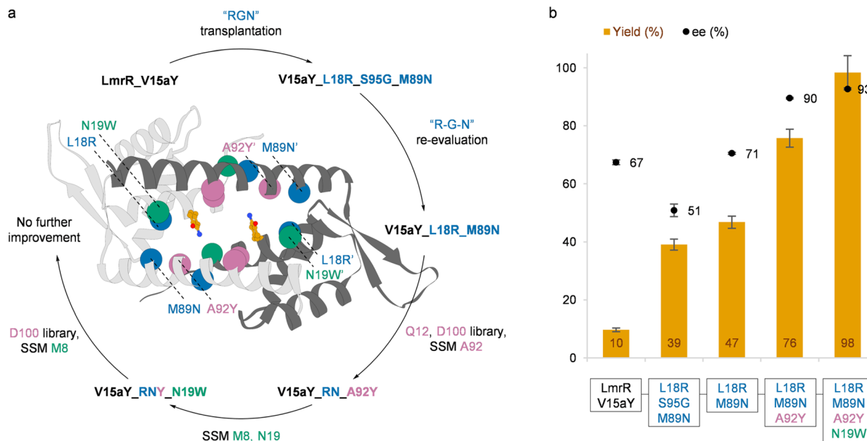
Fig. 1 Directed evolution of V15aY for the enantioselective vinylogous FC-alkylation of 2a with 1a . (a) Trajectory of the directed evolution campaign. Positions targeted in each round are displayed as correspondingly coloured spheres in the crystal structure of LmrR_V15aY_RNYW (PDB 9H88), with the \alpha Y side chain displayed in orange. (b) Analytical yield and ee of the FC-alkylation reaction between 1a and 2a to give 3a for the different variants obtained during directed evolution, using 60 \mu M protein at pH 5.5 (see Table 1 for reaction conditions). Results are based on at least three experiments, using two or more independently produced batches of protein. Errors are the standard deviation of the results.
