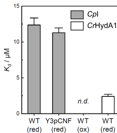
Fig. 6 Microscale thermophoresis. Dissociation constants ( K_d ) of the CpFd : CpI (WT) and Y3pCNF- CpFd : CpI complex under reducing or oxidizing conditions (red/ox). Under oxidizing conditions in the absence of dithionite, an interaction between CpFd : CpI was not detected (n.d.). The open bar depicts the K_d of the CpFd : CrHydA1 complex under reducing conditions. See Fig. S7† for the titration curves and additional data.
