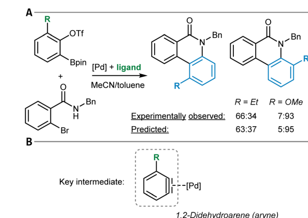
Fig. 18 (A) Palladium-catalyzed annulation of ortho -borylaryl triflates and the two possible reaction products with experimentally observed regioselectivities and the respective predictions from a linear model. The Hammett and Charton parameters of the R substituent and the cone angle of the applied ligand at palladium were used to predict regioselectivity. (B) The key intermediate of the reaction shown in (A), which is the palladium complex of the in situ -generated aryne.
