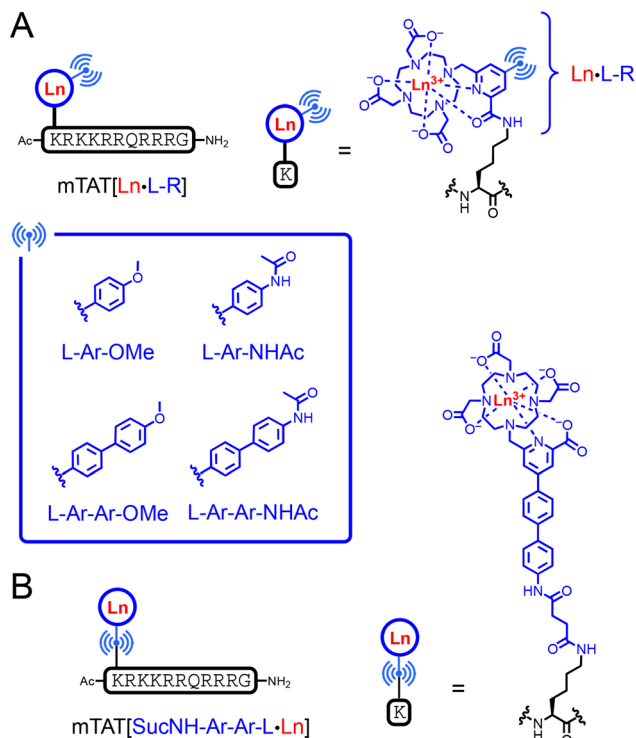
Fig. 2 Chemical structures of (A) mTAT[Ln \cdot L-R] conjugates ( R = Ar-OMe , Ar-NHAc , Ar-Ar-OMe and Ar-Ar-NHAc ; Ln = Eu^{3+} or Gd^{3+} ) and (B) the mTAT[SucNH-Ar-Ar-Ln] conjugate.
