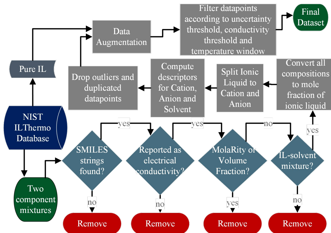
Figure 2: A brief illustration of the dataset formulation pipeline
