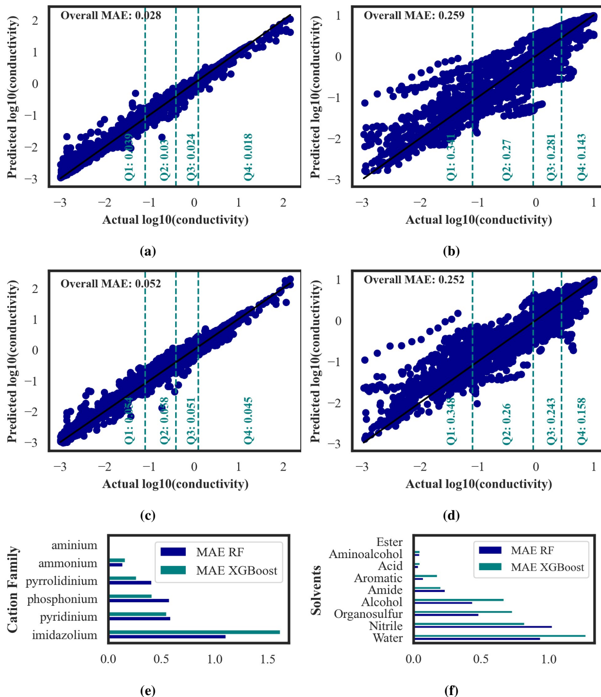
Figure 6: Performance analysis on stratified-IL split: (a) Random Forest, training dataset; (b) Random Forest, test dataset; (c) and (d) XGboost on training and test datasets, respectively. Figures (a)-(d) also include the information on the MAE for each of the quartiles. (e) and (f) depict MAE calculated for representative cation and solvent families, respectively.
