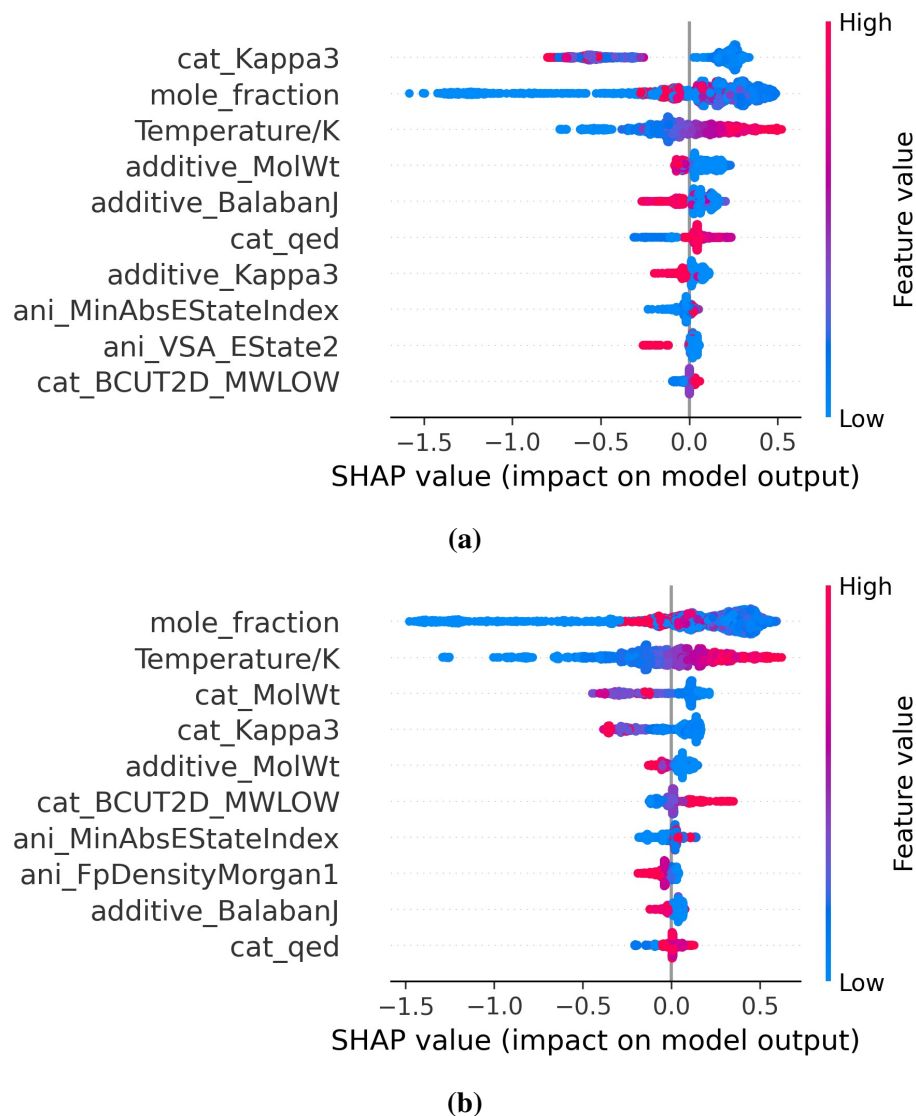
Figure 7: SHAP feature importance for (a) Random Forest and (b) XGBoost model
