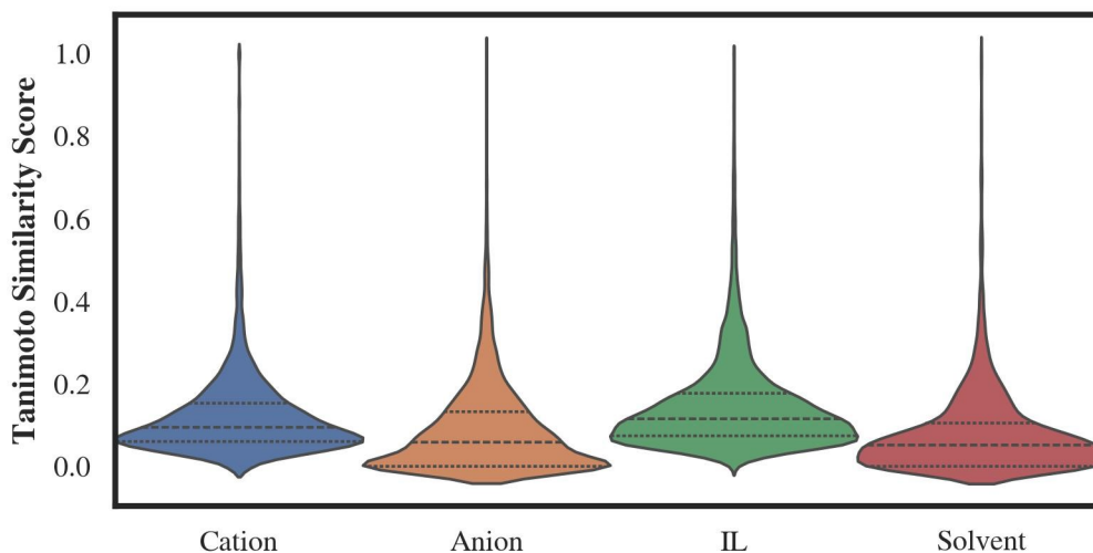
Figure 5: Tanimoto score distribution of cation, anions, ILs, and solvents in the dataset; the three dotted lines inside each of the violins represents quartiles.
