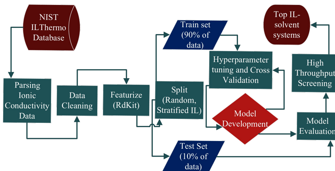
Figure 1: General workflow of our work
