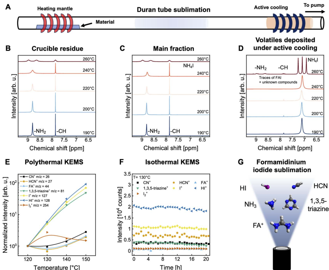
Fig. 2 Investigation of the thermal stability of FAI under sublimation conditions. (A) Schematic drawing of the employed sublimation setup. Material is collected from the crucible residue, main fraction, and the volatiles deposited under active cooling. (B–D) ^1\text{H} -NMR spectra of collected material for increasing sublimation temperatures (E) KEMS measurements of pristine FAI with increasing temperature. Lines are guides for the eye. (F) Isothermal KEMS measurements at 130^\circ\text{C} . (G) Graphical summary of species emitted from the sublimation source.
