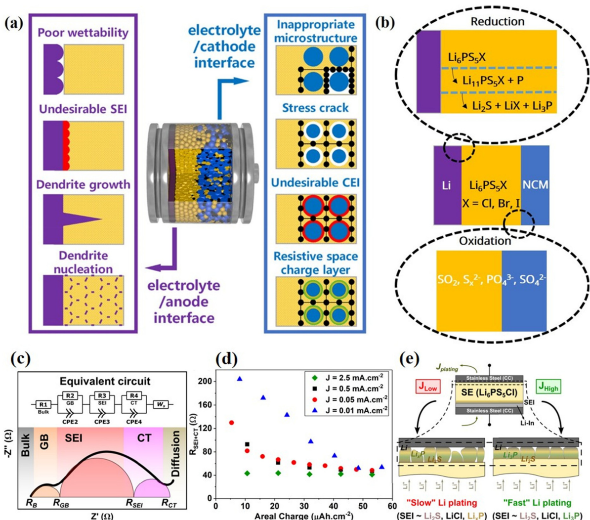
Fig. 1 (a) Challenges of SE and electrode interfaces in ASSLBs. 52 (b) Scheme illustrating the oxidation and reduction of \text{Li}_6\text{PS}_5\text{X} ( \text{X} = \text{Cl, Br, I} ) argyrodite SEs when in contact with electrodes during cycling. Interpretation of EIS spectra. (c) Equivalent circuit used for fitting the EIS data along with a schematic describing the impedance contributions from the bulk ( R_B ), grain boundaries ( R_{GB} ), SEI ( R_{SEI} ) and charge transfer ( R_{CT} ) processes. 46,47 (d) Variation in interfacial resistance, R_{\text{int}} (R_{\text{SEI}} + R_{\text{CT}}) , from fitted EIS data as a function of the amount of charge passed during Li plating at current densities, J_{2.5} = 2.5 \text{ mA cm}^{-2} , J_{0.5} = 0.5 \text{ mA cm}^{-2} , J_{0.05} = 0.05 \text{ mA cm}^{-2} and J_{0.01} = 0.01 \text{ mA cm}^{-2} . 46,47 (e) Schematic representation of the likely mechanism of SEI formation and Li plating as a function of applied current density, at J_{2.5} ( J_{\text{High}} ) and J_{0.01} ( J_{\text{Low}} ). 45
