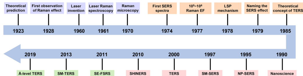
Fig. 2 A timeline of historical advances in Raman effect, SERS, and related revolutionizing science and technologies. The invention and introduction of the lasers in the 1960s expanded the applications of Raman spectroscopy. Advancements in nanoscience in the 1990s boosted the second upsurge of the SERS field. EF: enhancement factor; LSP: localized surface plasmon; NP: nanoparticle; SM: single-molecule; TERS: tip-enhanced Raman spectroscopy; SHINERS, shell-isolated nanoparticle-enhanced Raman spectroscopy; SE-FSRS: surface-enhanced femtosecond stimulated Raman spectroscopy.
