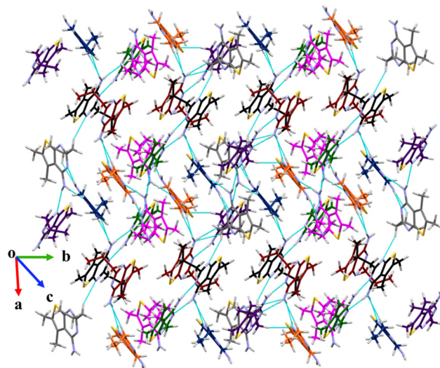
Fig. 5 Crystal packing depicts the crystalline arrangement of eight molecules through N-H \cdots N and C-H \cdots N interactions in compound 4 .
