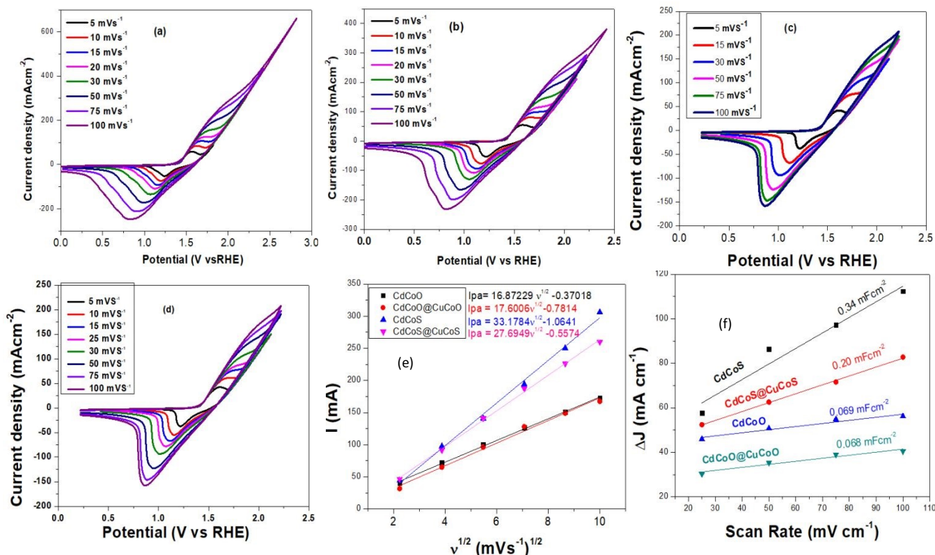
Figure 5. Cyclic voltammograms (CV) of the catalysts (a) CdCoS, (b) CdCoS@CuCoS, (c) CdCoO and CdCoO@CuCoO. The plot between the anodic peak current (Ipa) of cyclic voltammograms in 1.0 M KOH and the square root of the scan rates (v 1/2 ) for all as-synthesized catalysts.
