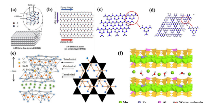
Fig. 2 (a) Layered van der Waals structure of bulk h-BN and (b) planar view of an atomically thin sheet of sp^2 -bonded B and N atoms that comprise the h-BN crystal or BN nanosheets (BNNS). Adapted with permission. 33 Copyright 2012, The Royal Society of Chemistry. Stacking 2D layering composition and fundamental constituent elements of (c) s-triazine and (d) tri-s-triazine of g-C 3 N 4 . 34 Copyright 2017, Elsevier. (e) Schematic representation of the structure of MMT. 35 Copyright 2021, Multidisciplinary Digital Publishing Institute. (f) Schematic diagram of VMT structure. 19 Copyright 2021, Elsevier.
