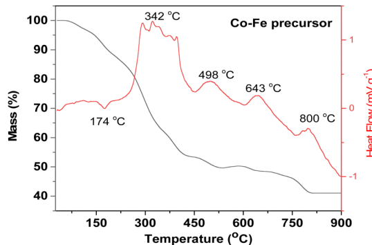
Fig. 2 Thermogravimetric (TGA) curve for the Co-Fe precursor.
