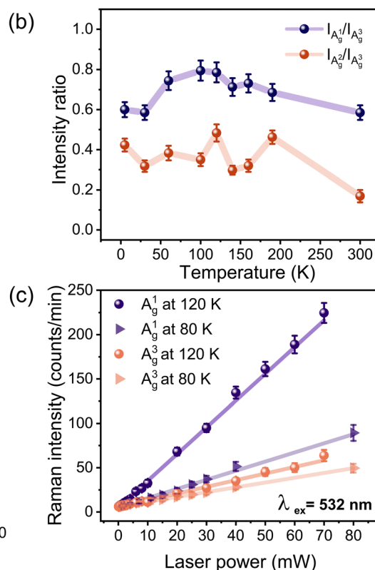
Fig. 5 (a) Temperature-dependent Raman spectra of bulk PdSe 2 under parallel configuration (xx) with an excitation energy of 2.52 eV (491 nm). (b) The intensity ratio of the Raman A g 1 and A g 2 to A g 3 mode. (c) Power dependence of the Raman intensities of the A g 1 and A g 3 phonon modes for 2.33 eV (532 nm) excitation energy and fixed temperatures of 120 and 80 K. The slope values of the A g 1 and A g 3 at 120 K and 80 K are 3.19, 1.11, 0.76 and 0.54 counts min -1 mW -1 , respectively.
