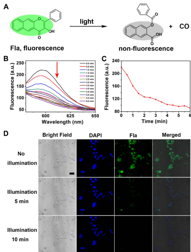
Fig. 3 (A) The schematic CO-releasing reaction of Fla. (B) Emission spectra of Neu-MOF/Fla ( 50 \mu\text{g mL}^{-1} ) with light illumination for 6 min. (C) Linear curves of photo-induced emission changes in Neu-MOF/Fla ( 50 \mu\text{g mL}^{-1} ). The emission wavelength being monitored was 596 nm. (D) Fluorescence images of BV2 cells exposed to Neu-MOF/Fla ( 50 \mu\text{g mL}^{-1} ) with light illumination for different times. Scale bar = 25 \mu\text{m} .
