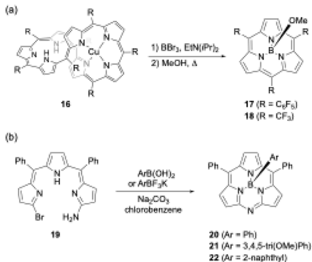
Scheme 4 (a) Metathesis-like ring splitting of heptaphyrin 16 , and (b) boron-templated synthesis of submonoozaporphyrins.
