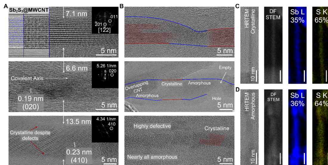
Fig. 3 Sb 2 S 3 encapsulated within MWCNTs. (A) Representative HRTEM of crystalline Sb 2 S 3 @MWCNTs. The topmost image contains a model (left), simulated image (middle), and real image (right). For all three images, the corresponding FFT of the micrographs are located on the top-right panel. (B) Representative HRTEM of amorphous a-Sb 2 S 3 @MWCNTs. The crystalline domains of c-Sb 2 S 3 are highlighted in red for easier visualization, while the a-Sb 2 S 3 domains are highlighted in blue. (C) EDS map of a c-Sb 2 S 3 nanowire bundle encapsulated within a MWCNT. (D) EDS map of an amorphous a-Sb 2 S 3 nanowire within a MWCNT.
