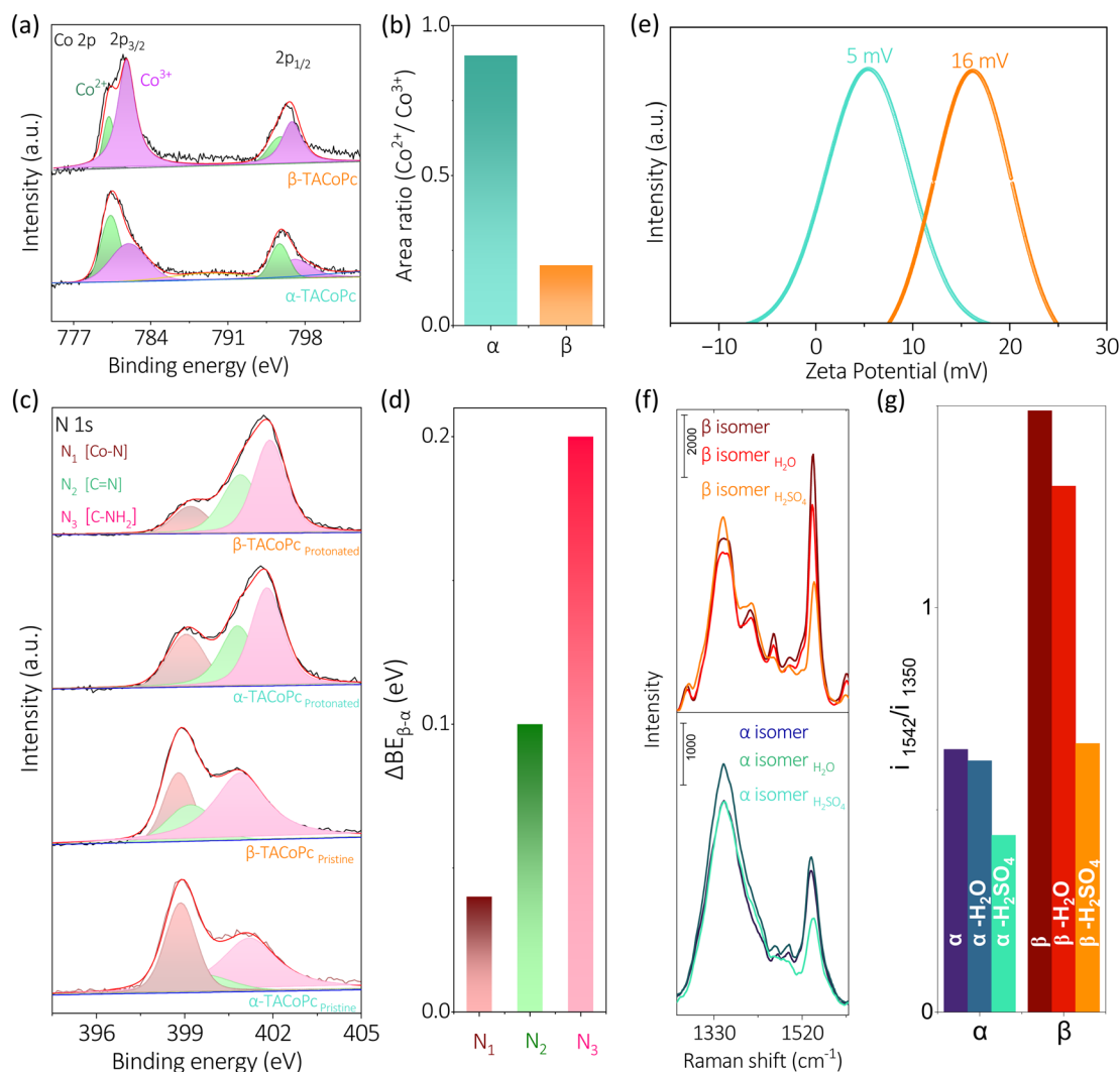
Fig. 4 (a) Co 2p XPS spectra of \alpha -TACoPc and \beta -TACoPc molecules. (b) Co^{2+}/Co^{3+} area ratio which is extracted from (a). (c) N 1s XPS spectra of (c) pristine and protonated forms of \alpha -TACoPc and \beta -TACoPc isomers. (d) Bar plot showing the difference of N 1s binding energies between protonated \beta -TACoPc and protonated \alpha -TACoPc molecules ( \Delta BE_{\beta-\alpha} ). (e) Zeta potential profiles of \alpha -TACoPc and \beta -TACoPc isomeric molecules. (f) Raman spectra of \alpha -TACoPc (bottom panel) and \beta -TACoPc (top panel) isomers and (g) the intensity ratio of i_{1542}/i_{1350} peaks in the absence and presence of various solvents.
