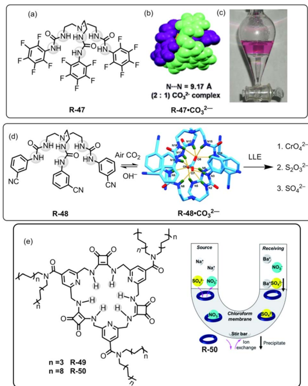
Fig. 16 (a) Chemical structure of the receptor R-47. (b) Representation of the assembly of R-47 \cdot CO_3^{2-} . (c) Visualization of SO_4^{2-} extraction using phenolphthalein through the R-47 \cdot CO_3^{2-} complex. (Reproduced from ref. 81. Copyright 2012, The Royal Society of Chemistry.) (d) Schematic representation of LLE by R-48 (Reproduced from ref. 82. Copyright 2014, Wiley.) (e) Chemical structures of the receptors R-49 and R-50. Illustration of the general setup for the U-tube experiments used to test the ability of R-50 to act as a carrier for SO_4^{2-} . (Reproduced from ref. 83. Copyright 2020, The Royal Society of Chemistry.)
