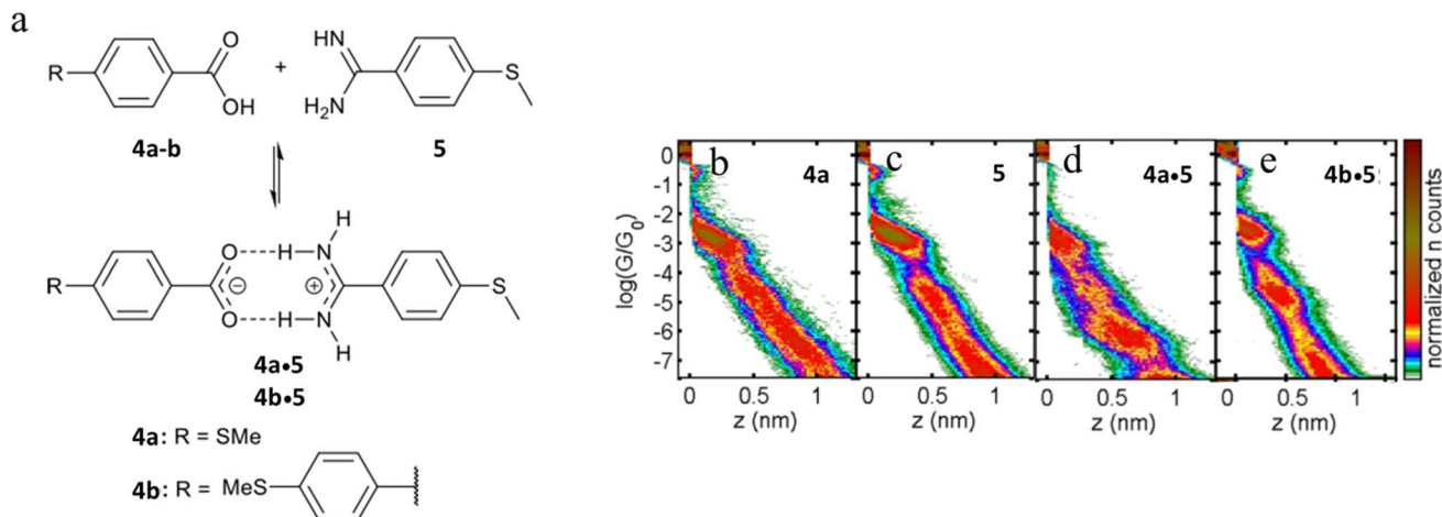
Fig. 23 (a) Supramolecular H-bonded amidinium-carboxylate wires ( 4a·5 and 4b·5 ); 2D conductance histograms for (b) 4a , (c) 5 , (d) complex 4a·5 , (e) complex 4b·5 . Figures adapted with permission from ref. 102. Copyright 2020, American Chemical Society.
