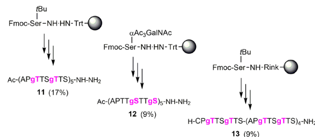
Scheme 3 Solid-phase synthesis of MUC5AC glycopeptides and their yields after isolation in parentheses. gS, gT = Ser/Thr( \alpha GalNAc). Conditions: Fmoc-cleavage: 20% piperidine in DMF; coupling: HATU/Oxyma/DiPEA (5 eq., 5 eq., 15 eq.); coupling of 7t or 7s: see condition 3, Table 5; capping: Ac 2 O/DiPEA/DMF (70 : 20 : 10, v/v/v); TFA cleavage: for 11 and 12 TFA/TIS/H 2 O (96/2/2). For 13 TFA/TIS/EDT/H 2 O (94/2/2/2).
