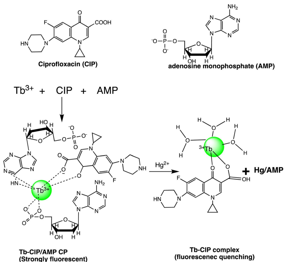
Scheme 24 Schematic representation of Tb-CIP/AMP CP preparation and Hg(II) sensing.
