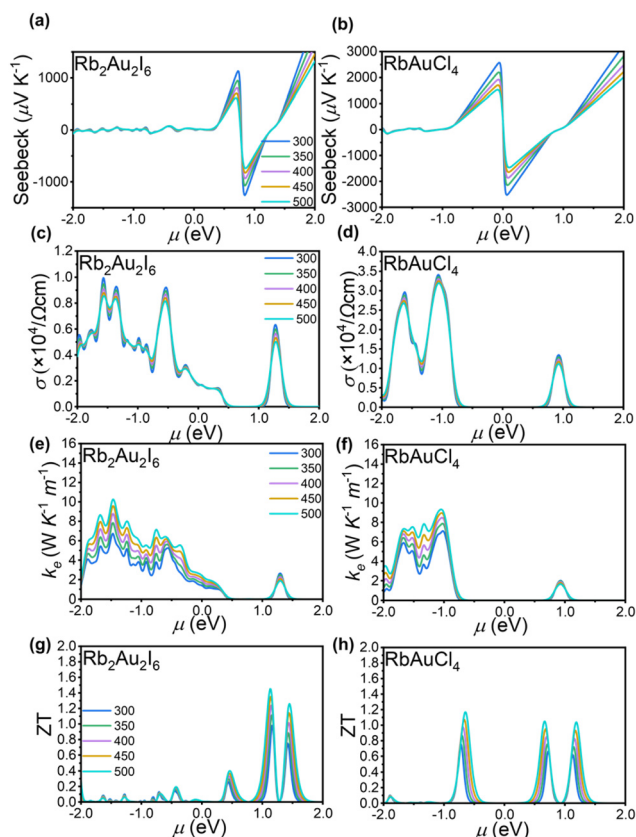
Fig. 5 (a and b) Dependence of chemical potential for \text{Rb}_2\text{Au}_2\text{I}_6 and \text{RbAuCl}_4 on the Seebeck coefficient; (c and d) electrical conductivity ( \sigma ); (e and f) temperature electronic thermal conductivity ( \kappa_e ); and (g and h) thermoelectric figure of merit ( ZT ) at different temperatures.
