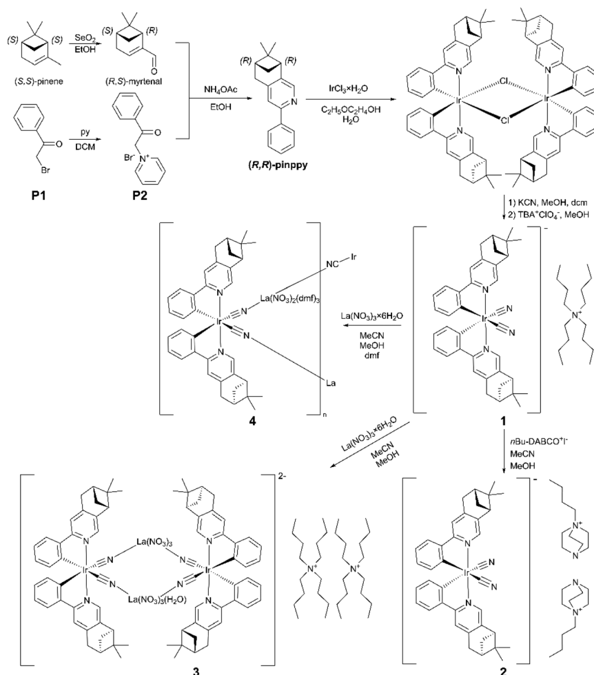
Scheme 1 Reported synthetic route for an enantiopure ( R,R )-pinppy ligand starting from ( S,S )-pinene and 2'-bromoacetophenone ( P1 ), and further syntheses of compounds 1–4 which are based on chiral dicyanidoiridate(III) complexes bearing the deprotonated form of ( R,R )-pinppy. In all cases, the chirality at the ligand is of the ( R,R )-type, whereas the detected diastereoisomers related to the chirality at the metal differ, i.e., the \Delta -isomers are present for 1 and 2 , while the \Lambda -isomers are observed in 3 and 4 . They are properly visualized in this scheme (see the text for details).
