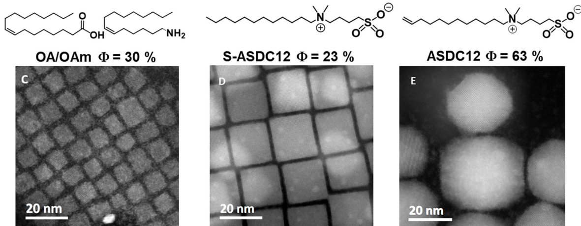
Fig. 5 Absorbance (A) and PL (B) spectra of CsPbBr 3 NCs capped with OA/OAm, and (C)–(E) HAADFpn images and their respective PLQY ( \Phi ).
